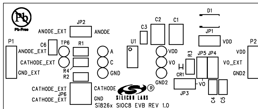
Figure 8. Si826x SOIC8 Evaluation Board Silkscreen
